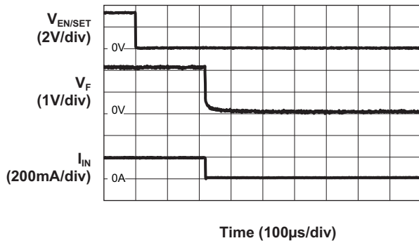
Turn-Off from 1.5x Mode Backlight ( V_{IN} = 3.6V ; 30mA/Channel; Fade-In/Out Disabled)
