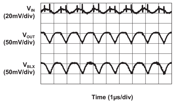
Backlight Operating Characteristics ( V_{IN} = 3.6V ; 1.5x Mode; 30mA/Channel; AC Coupled)
