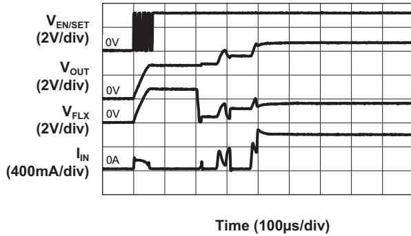
Turn-On to 2x Mode Flash ( V_{IN} = 2.8V ; 151mA/Channel)
