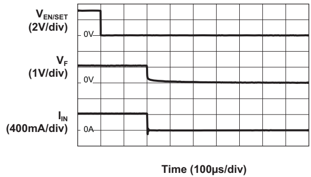
Turn-Off from 1.5x Mode Flash ( V_{IN} = 3.6V ; 151mA/Channel)
