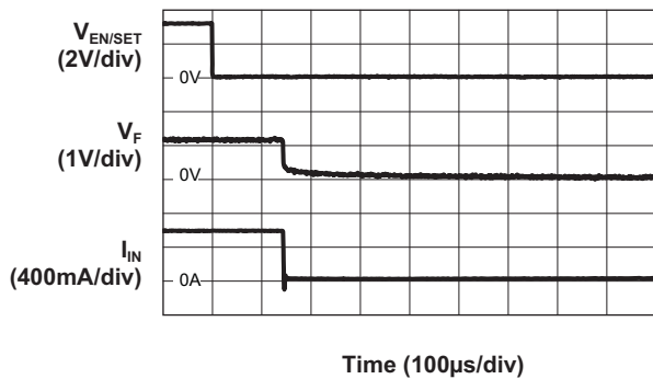
Turn-Off from 2x Mode Flash ( V_{IN} = 2.8V ; 151mA/Channel)
