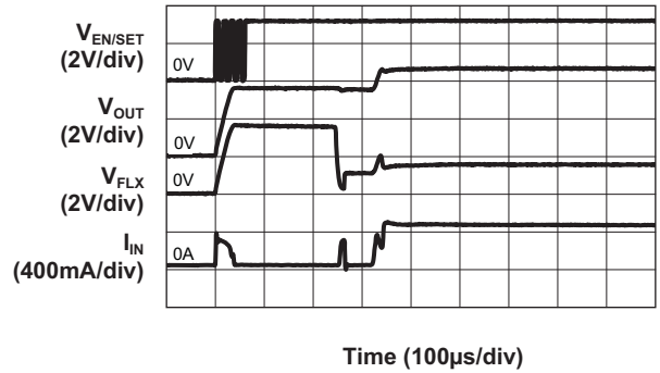
Turn-On to 1.5x Mode Flash ( V_{IN} = 3.6V ; 151mA/Channel)
